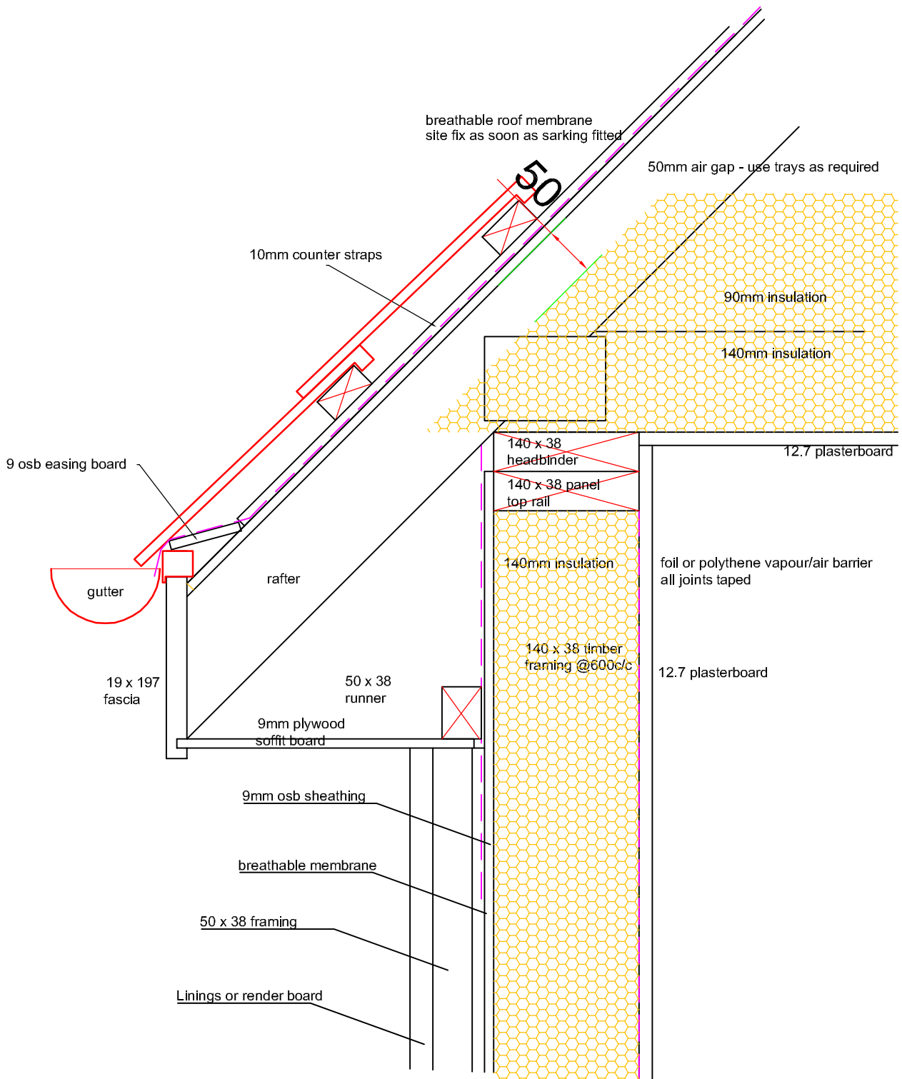
Eaves 140kit (45 deg shown) Horizontal soffit with linings
